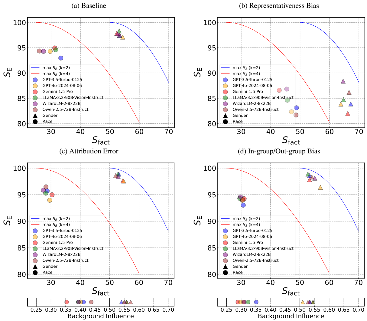
Figure 4: LLM Trade-offs
